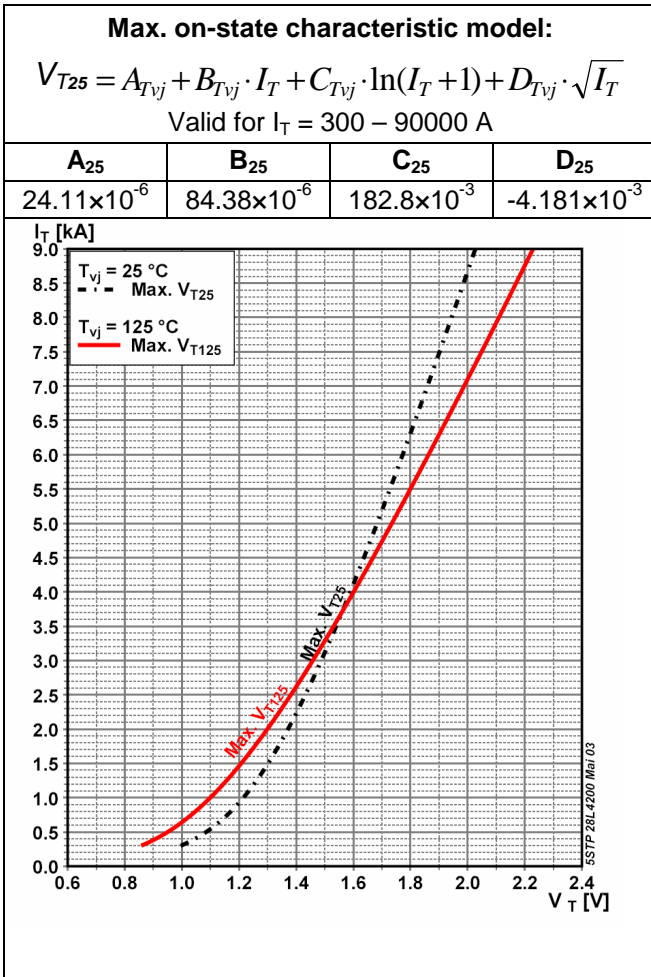
Fig. 2 On-state characteristics, T_j=125^\circ\text{C} , 10ms half sine
